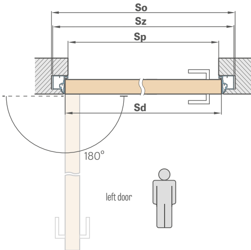
ALUMINIUM DOOR FRAME CROSS-SECTION
