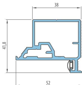
ALUMINIUM DOOR FRAME CROSS-SECTION
