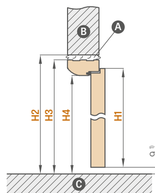
A-foam B-wall C-floor
