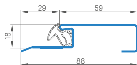
STAINLESS STEEL SHEET THRESHOLD
